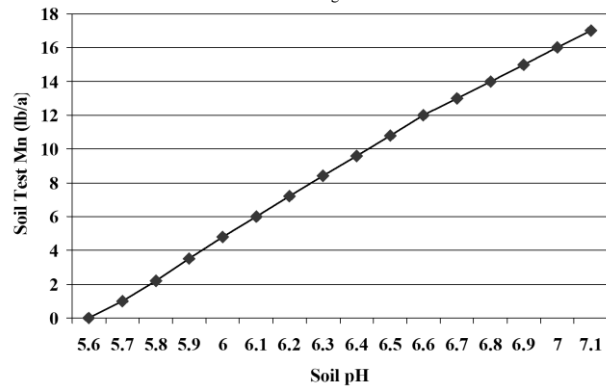
Figure 4. Relationship between pH and manganese availability. Maintain soil test manganese levels above the line to help avoid manganese deficiency. Source: Soil Test Handbook for Georgia.
